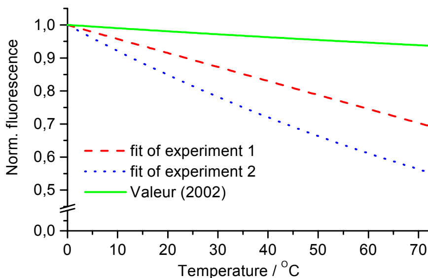
Figure 7: Fit of experimental data and theoretical values for intensity in relative units. Further explanations are given in the text.
