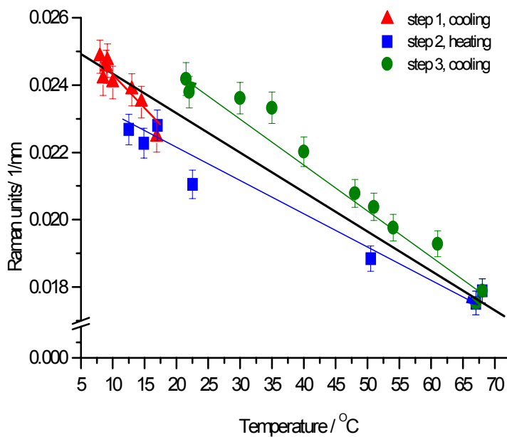
Figure 3: Temperature dependence of humic-type fluorescence intensity normalized by water Raman scattering. Different colours show steps of the experiment: cooling from room temperature to 6°C, heating up to 70°C, and then cooling back to room temperature.
