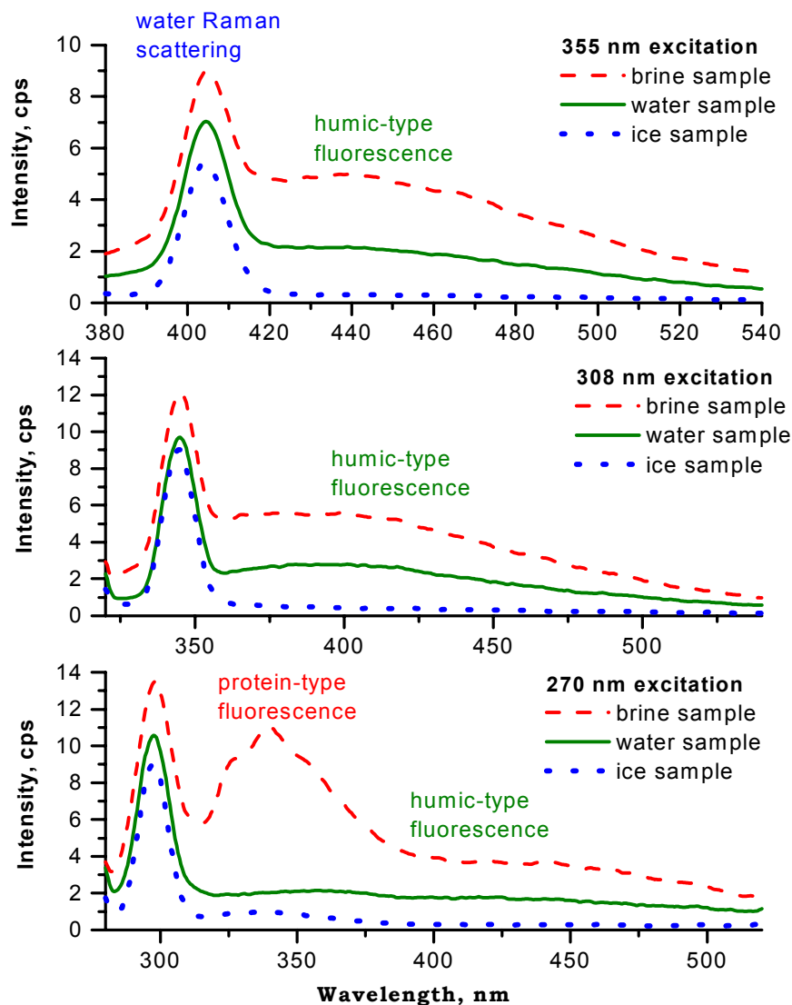
Figure 2: CDOM fluorescence spectra for samples taken at the end of the ARCTECLAB experiment.
