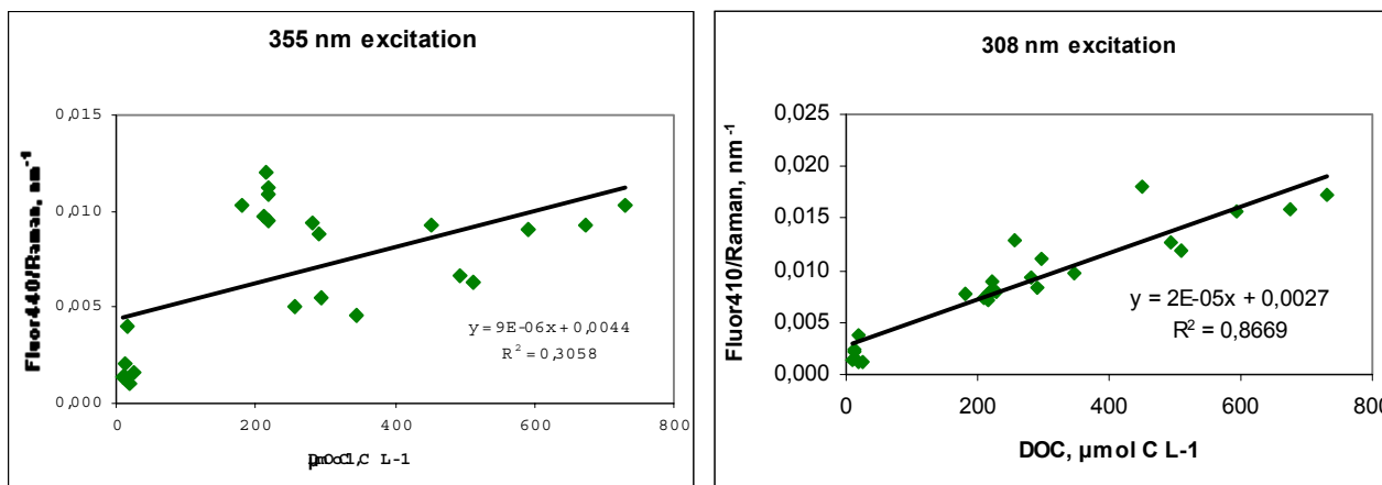
Figure 6. Fluorescence intensities versus DOC concentration for tank A, excitation at 355 and 308 nm.
