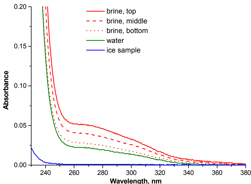
Figure 1: Absorbance spectra for samples taken at the end of the ARCTECLAB experiment. The optical path length is 1 cm.
