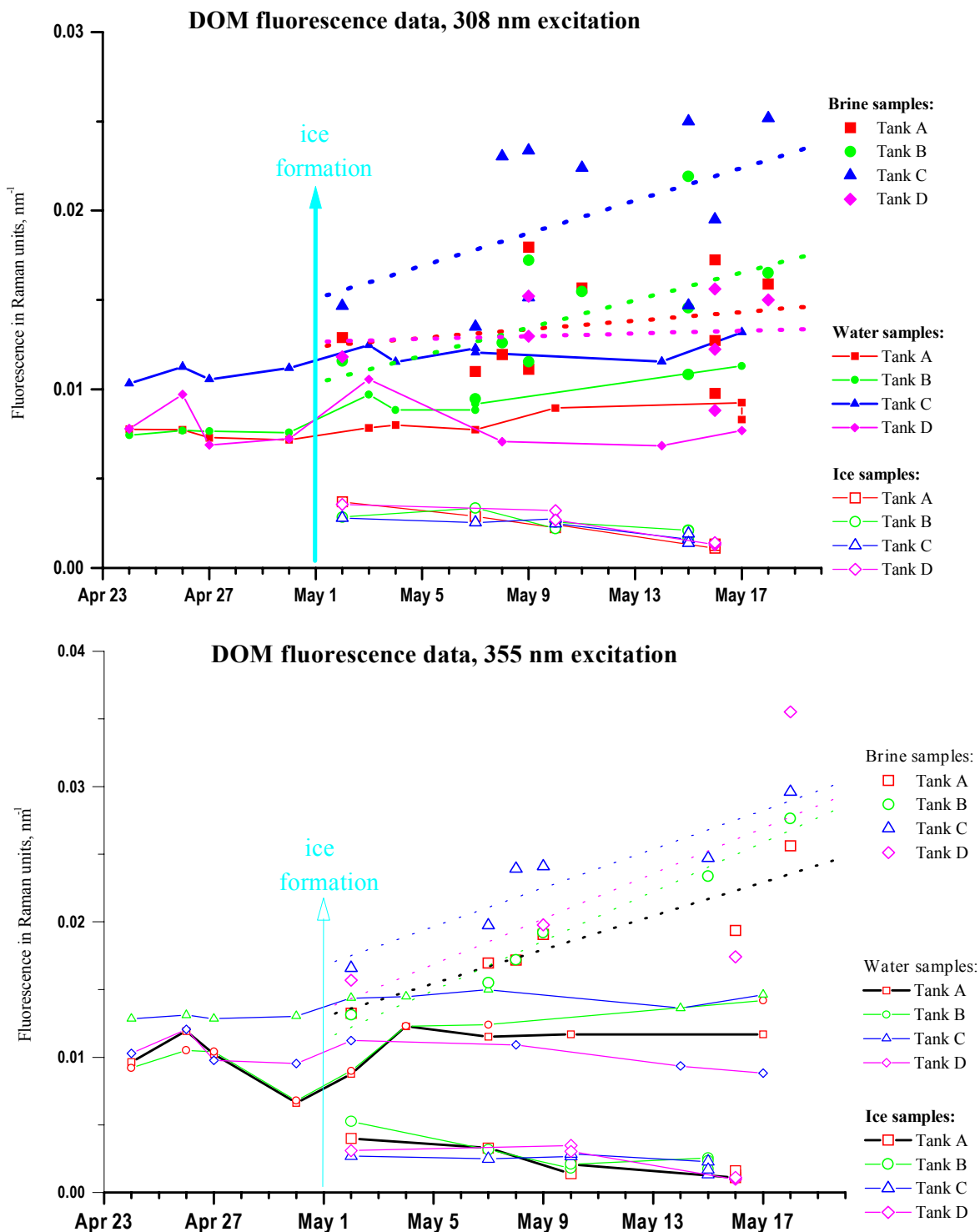
Figure 5. CDOM fluorescence intensities during the ARCTECLAB experiment. The date of ice formation is marked. 308 nm (top picture) and 355 nm excitation (bottom picture).
